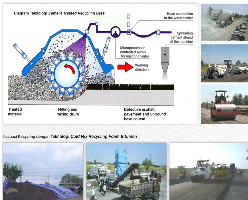
Gambar 6. Recycling asphalt pavement
